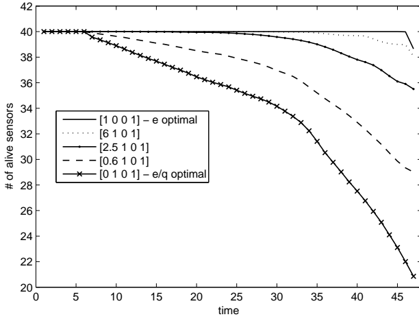
Fig. 3. Number of alive sensors for the e , eq and e/q -optimal SA strategies
