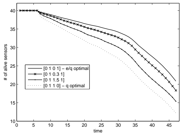
Fig. 2. Number of alive sensors for the q , qe and e/q -optimal SA strategies
