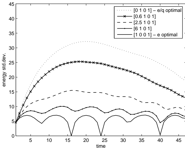
Fig. 4. Standard deviation of the residual energies for the q , qe and e/q -optimal SA strategies
