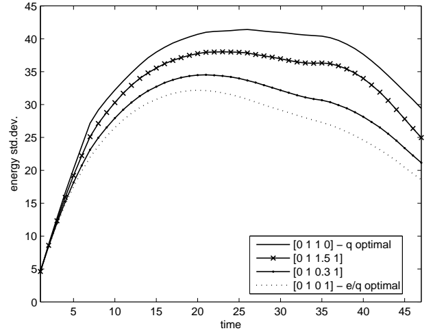
Fig. 5. Standard deviation of the residual energies for the e , eq and e/q -optimal SA strategies
