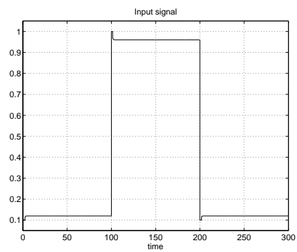
Figure 3: Saturated input
