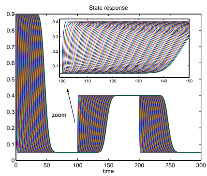
Figure 2: State response for 1 \leq i \leq n = 100
