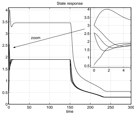
Figure 6: State response
