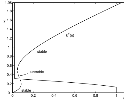
Figure 4: The intersection between the plant I/O characteristic k^Y(u) and u = \text{sat}(\ell(y, r)) for r = 0.3
