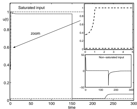
Figure 7: Saturated input (solid), \tilde{u}_{max}(t) and \tilde{u}_{min}(t) behaviour (dashed) in the main picture and the non-saturated input (solid) in the minor one
